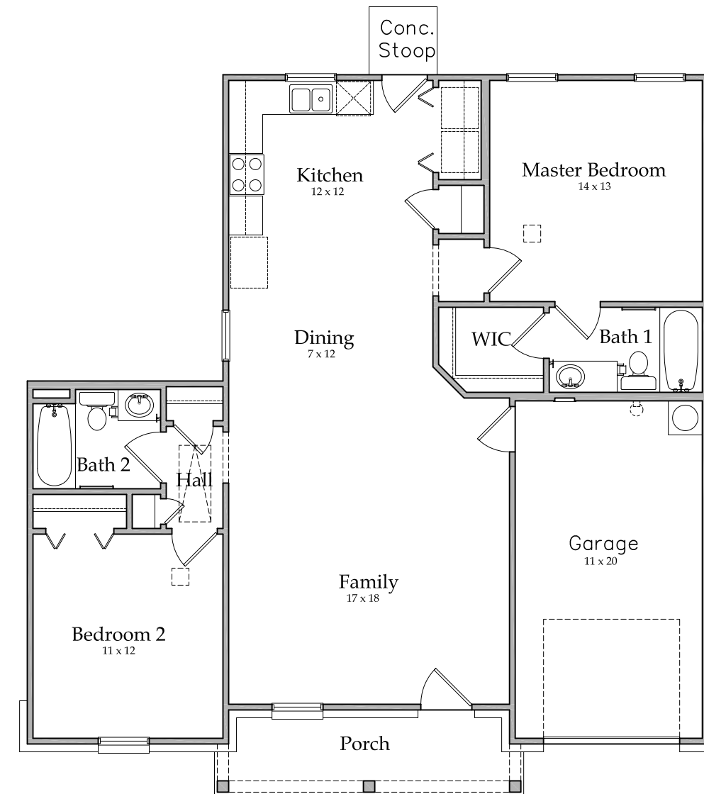
FLOOR PLAN
