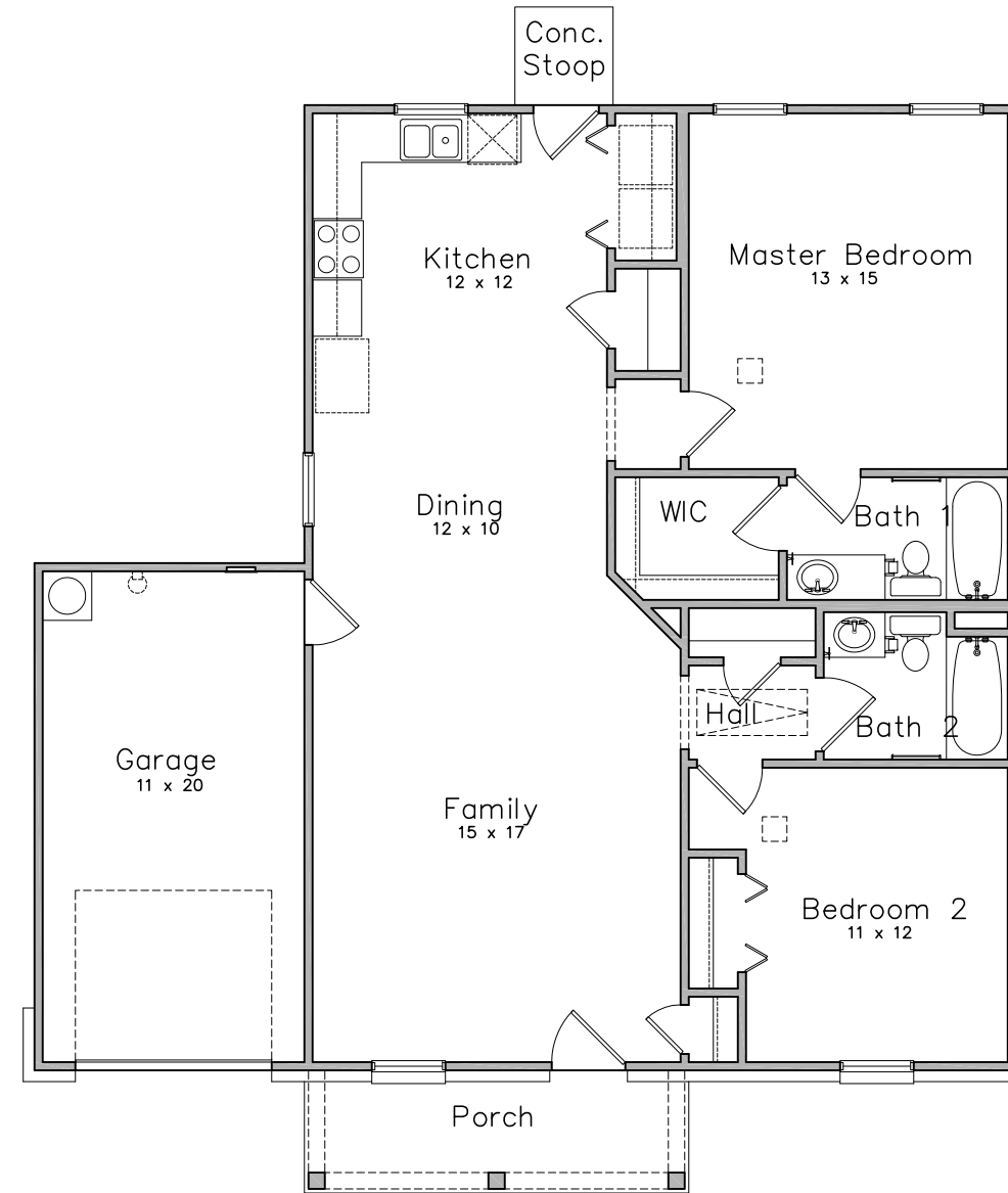
FLOOR PLAN
